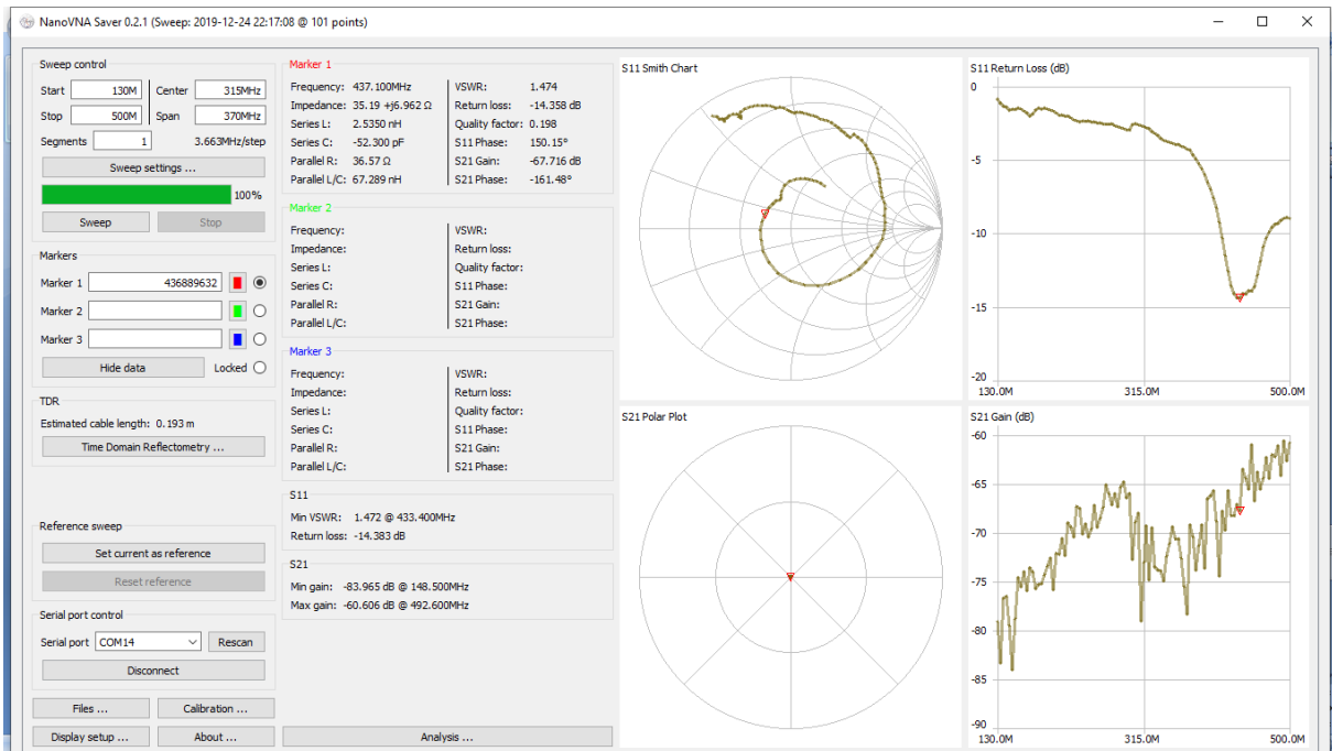
Monoband70cmb – zkracena 3cm
